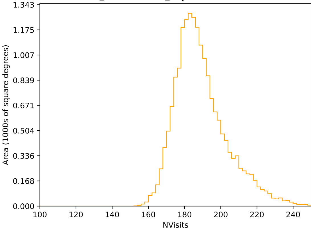
weather_cloudso0v3.4_10yrs WFD r band: NVisits
