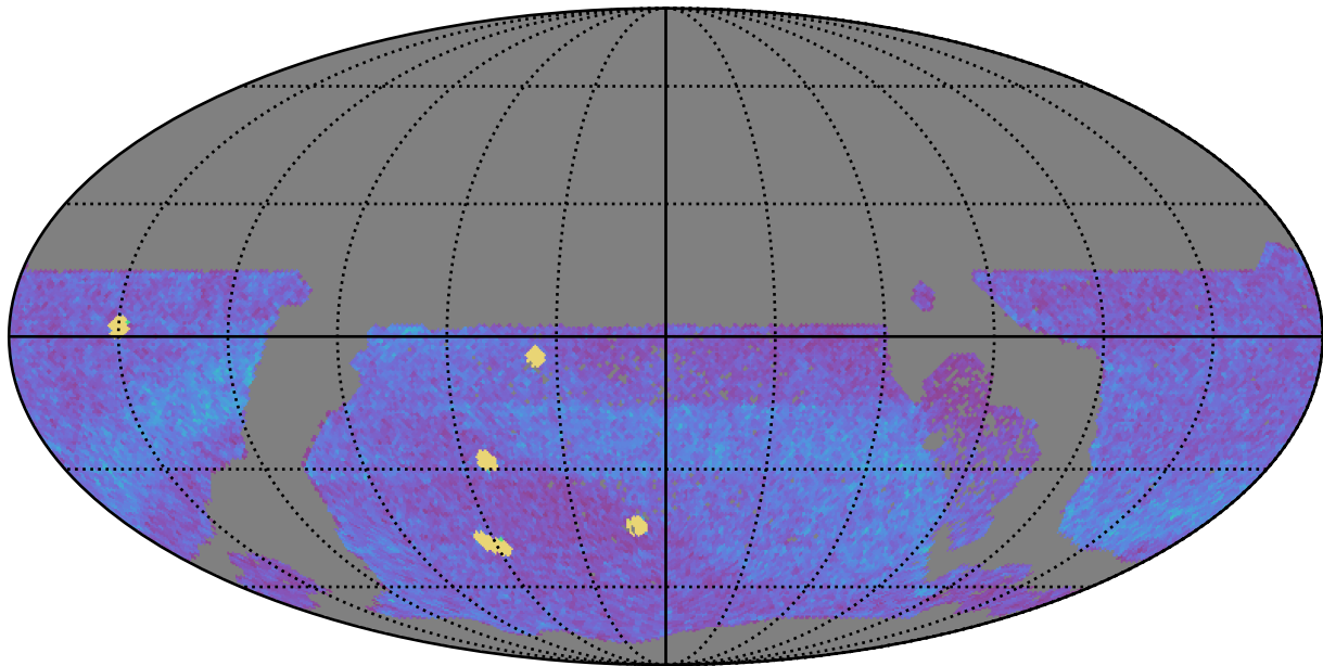
weather_cloudso0v3.4_10yrs WFD all bands: NVisits
