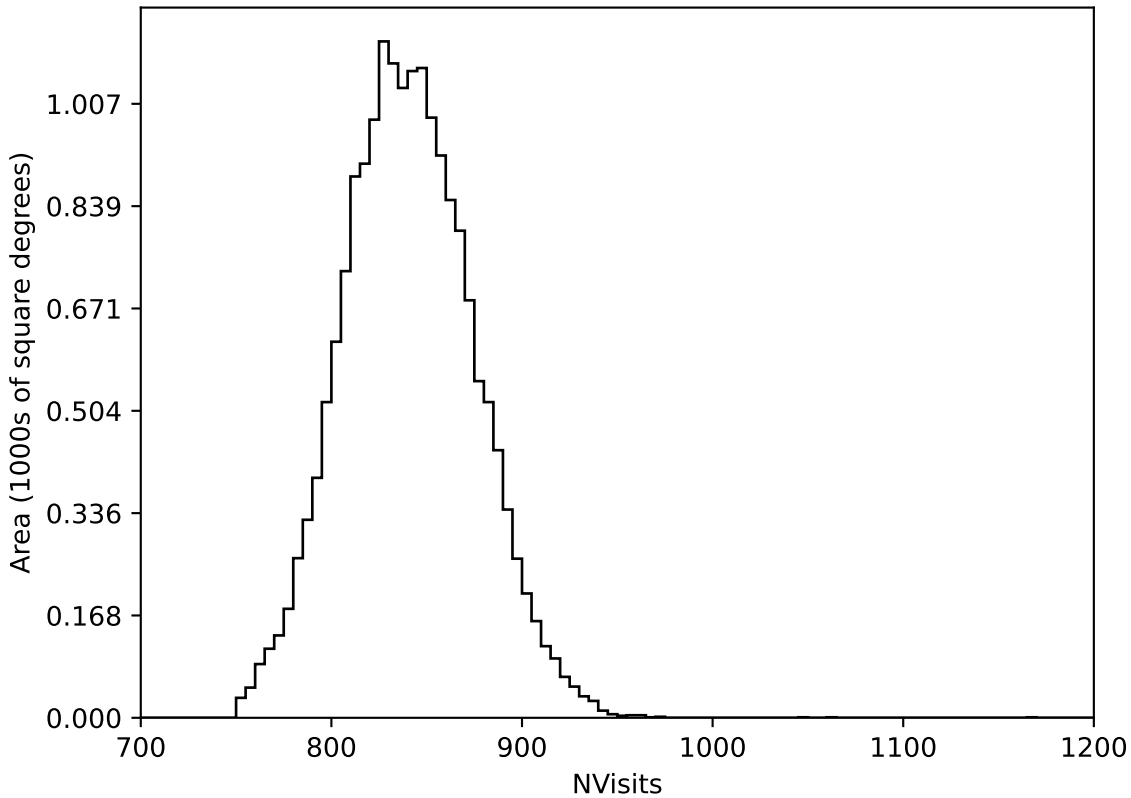
weather_cloudso0v3.4_10yrs WFD all bands: NVisits
