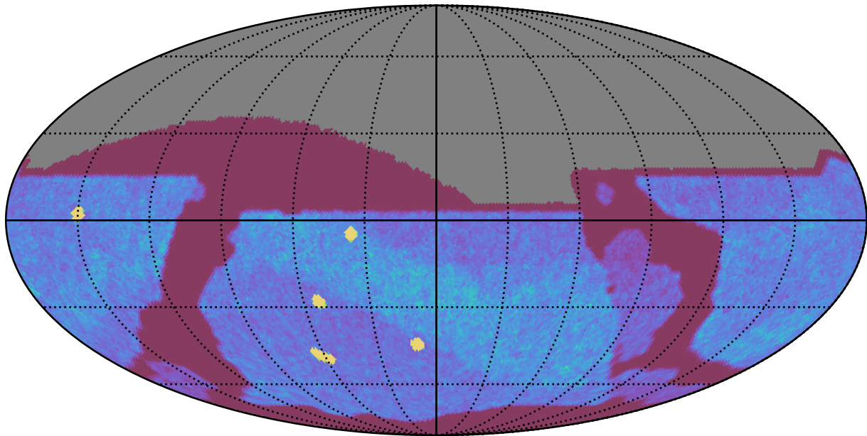
weather_cloudso0v3.4_10yrs All sky z band: NVisits
