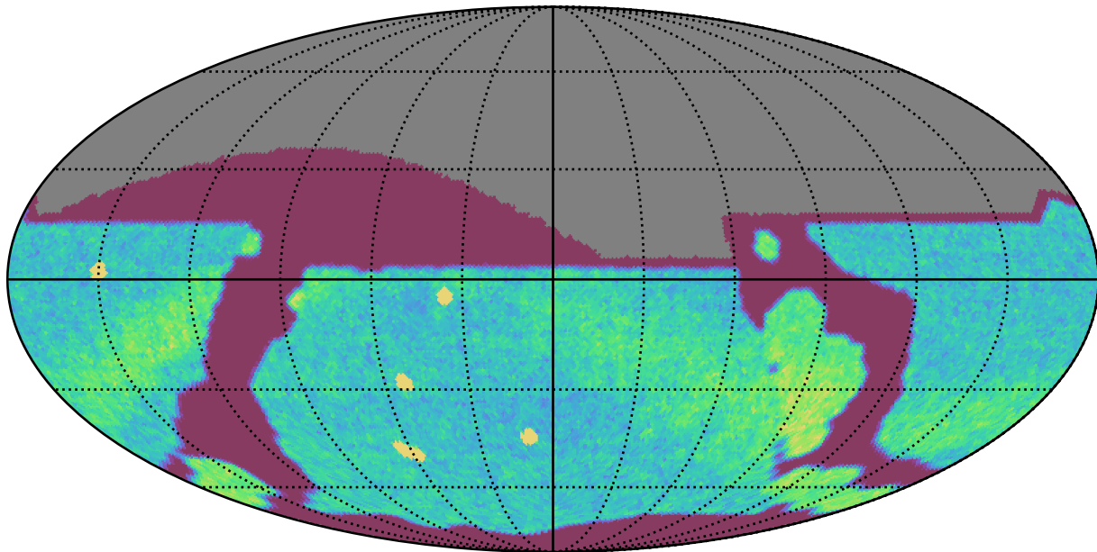
weather_cloudso0v3.4_10yrs All sky r band: NVisits
