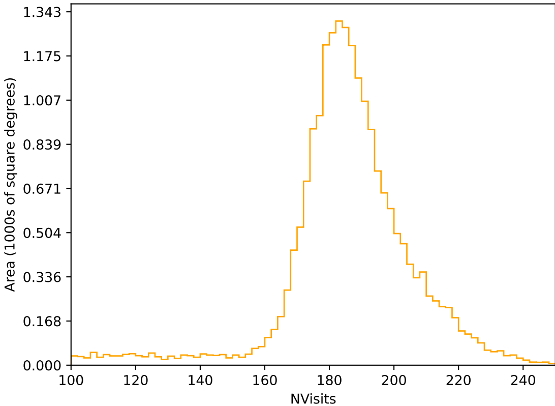
weather_cloudso0v3.4_10yrs All sky r band: NVisits
