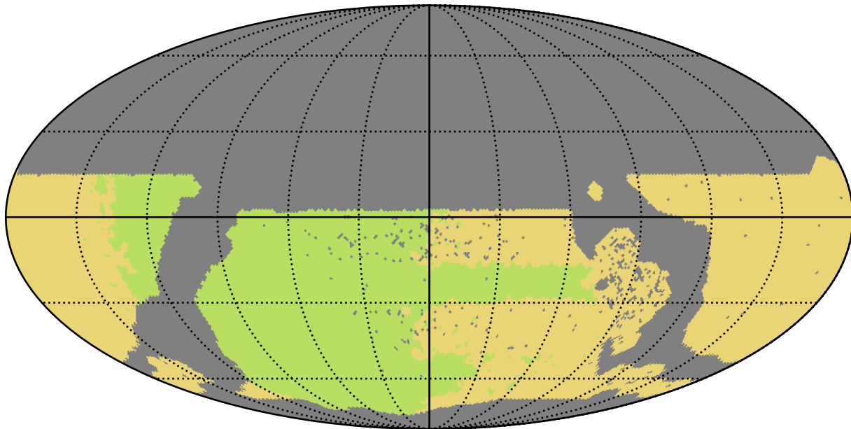
weather_cloudso0v3.4_10yrs WFD all bands: NSeasons
