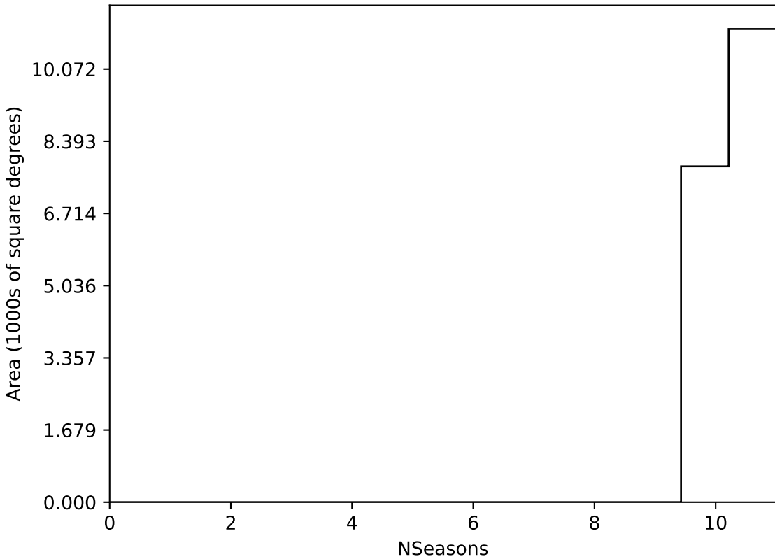
weather_cloudso0v3.4_10yrs WFD all bands: NSeasons
