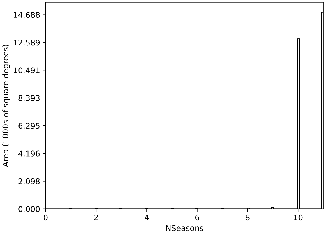
weather_cloudso0v3.4_10yrs All sky all bands: NSeasons
