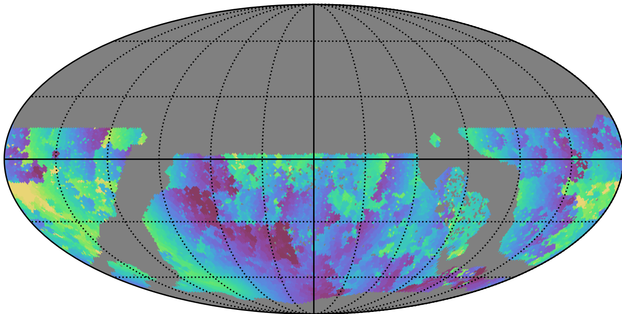
weather_cloudso0v3.4_10yrs WFD u band: Min solarElong
