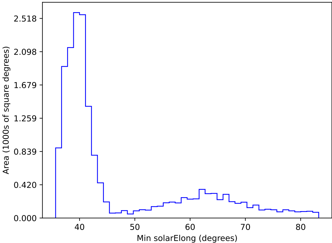
weather_cloudso0v3.4_10yrs WFD all bands: Min solarElong
