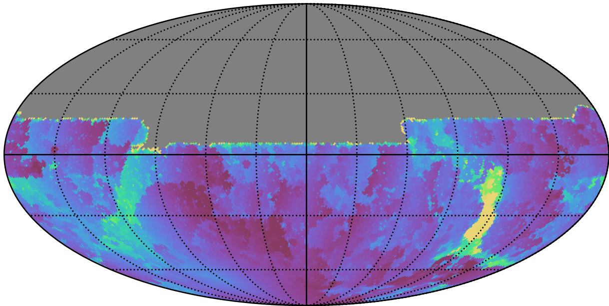
weather_cloudso0v3.4_10yrs All sky u band: Min solarElong
