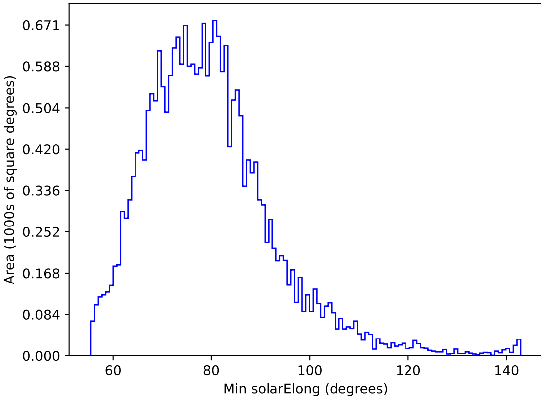
weather_cloudso0v3.4_10yrs All sky u band: Min solarElong
