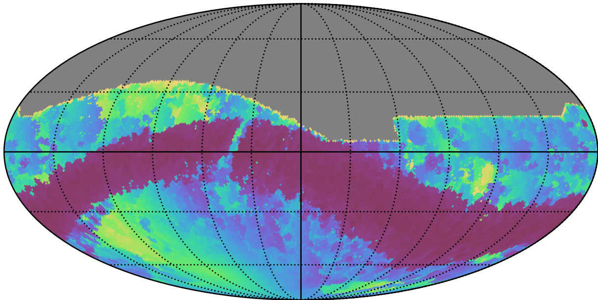
weather_cloudso0v3.4_10yrs All sky r band: Min solarElong
