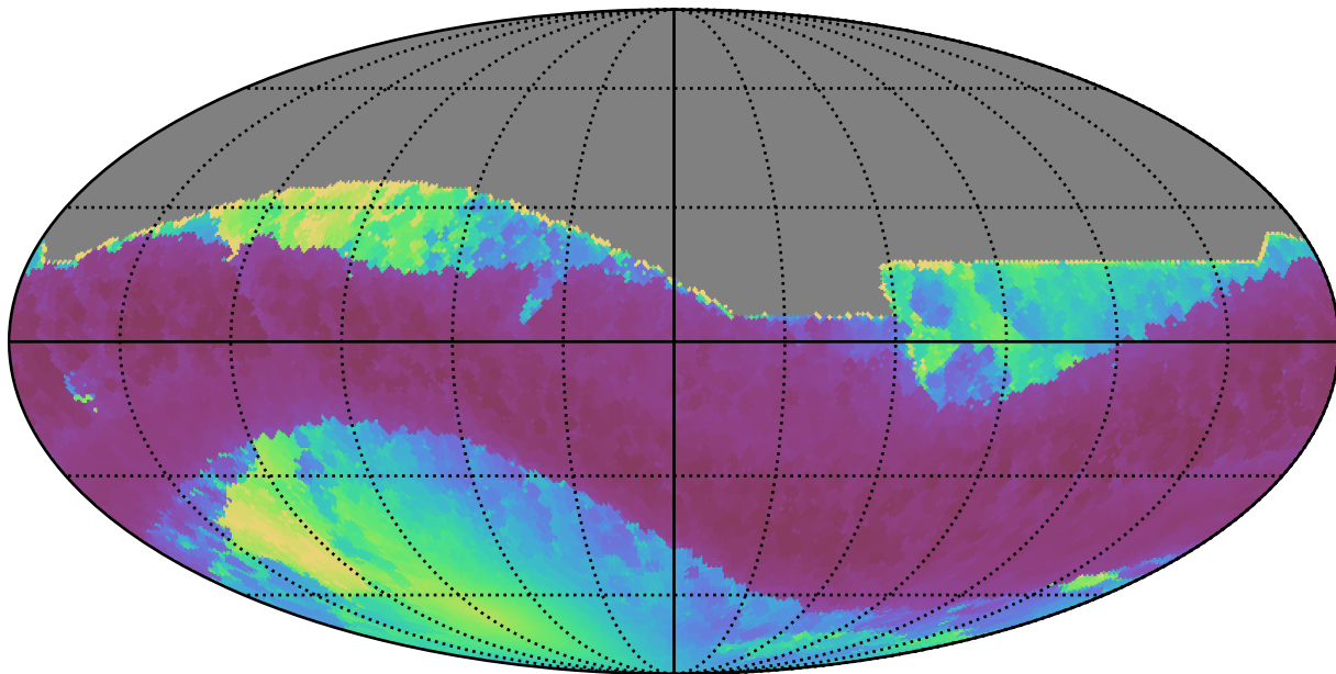
weather_cloudso0v3.4_10yrs All sky all bands: Min solarElong
