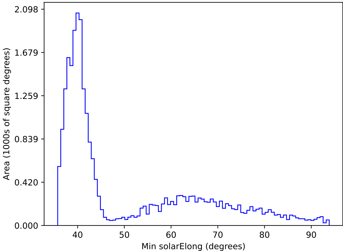
weather_cloudso0v3.4_10yrs All sky all bands: Min solarElong
