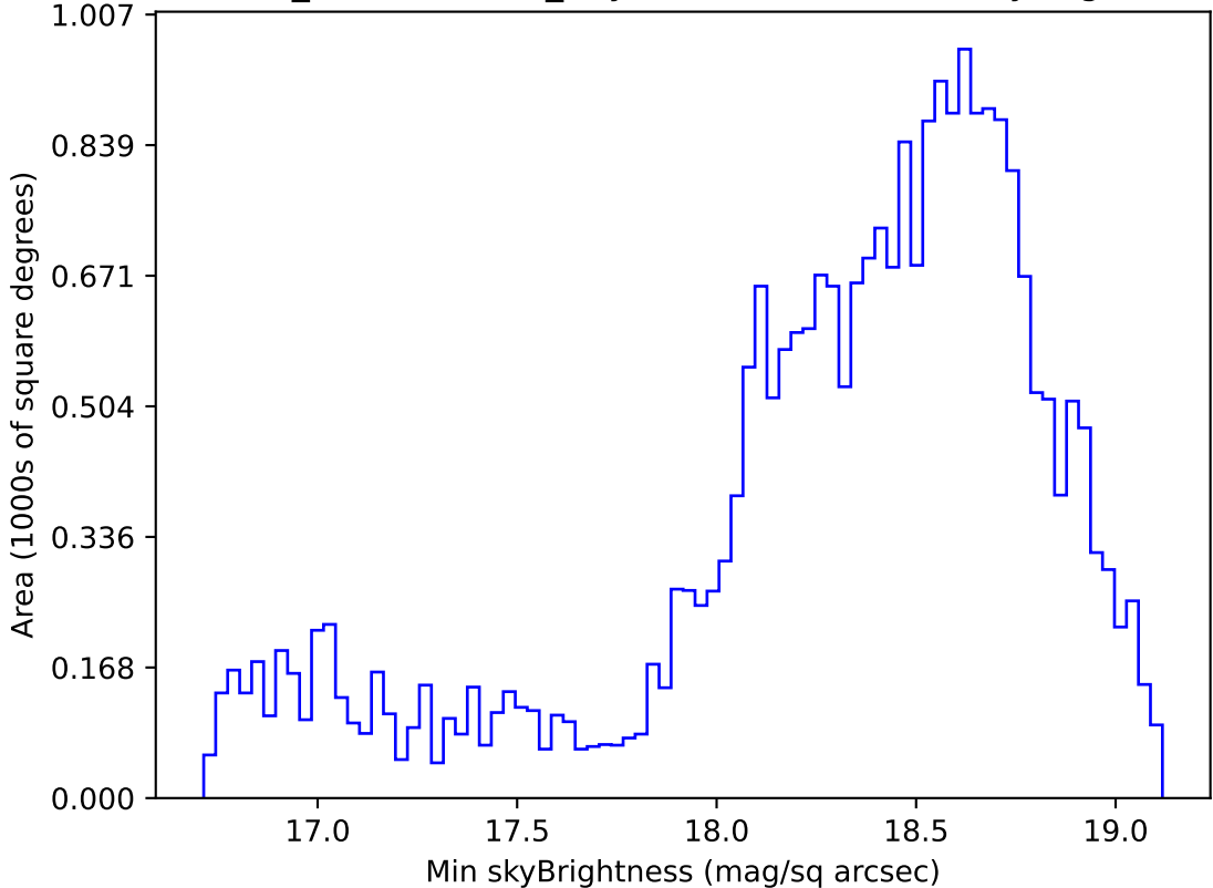
weather_cloudso0v3.4_10yrs Yr 1 z band: Min skyBrightness
