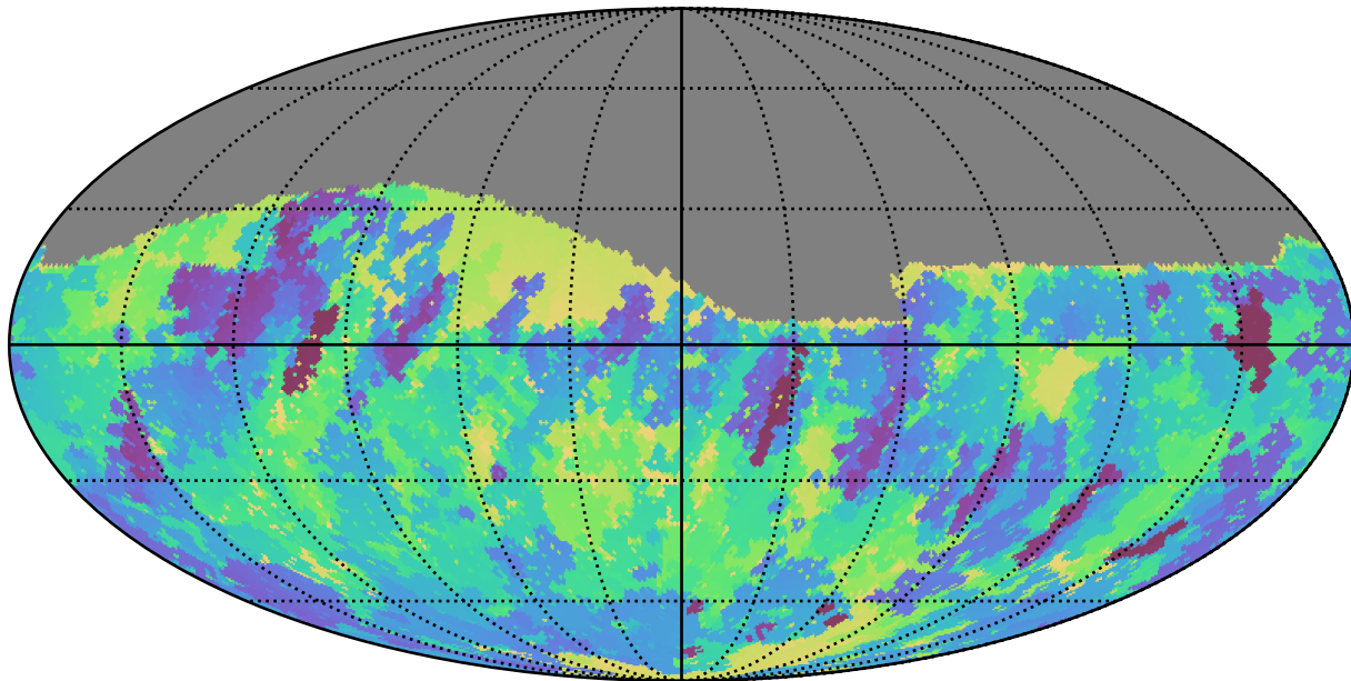
weather_cloudso0v3.4_10yrs Yr 1 r band: Min skyBrightness
