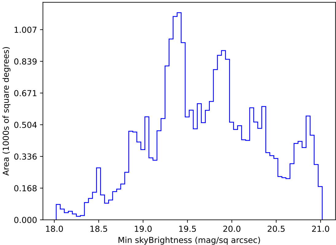
weather_cloudso0v3.4_10yrs Yr 1 r band: Min skyBrightness
