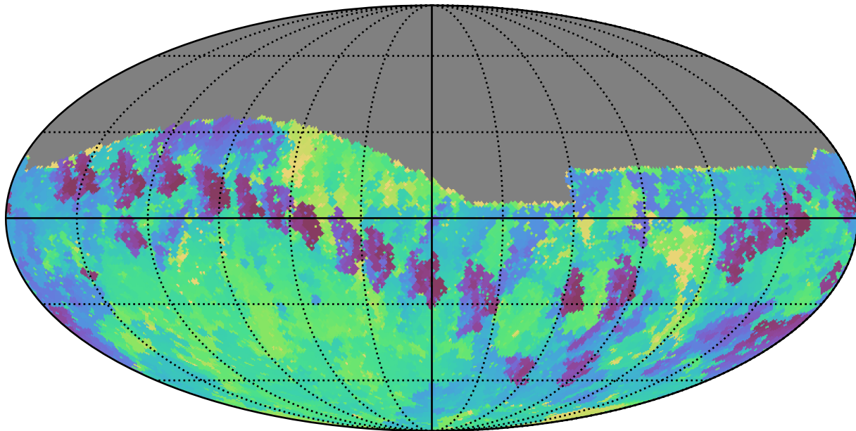
weather_cloudso0v3.4_10yrs Yr 1 i band: Min skyBrightness
