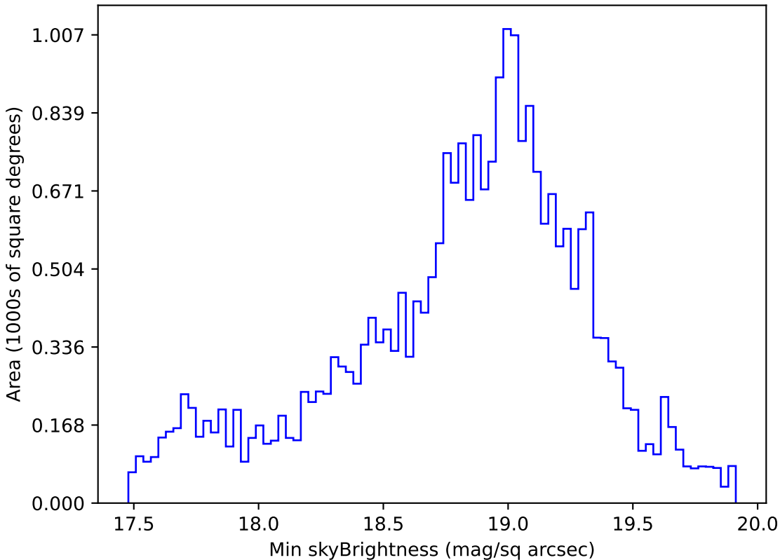
weather_cloudso0v3.4_10yrs Yr 1 i band: Min skyBrightness
