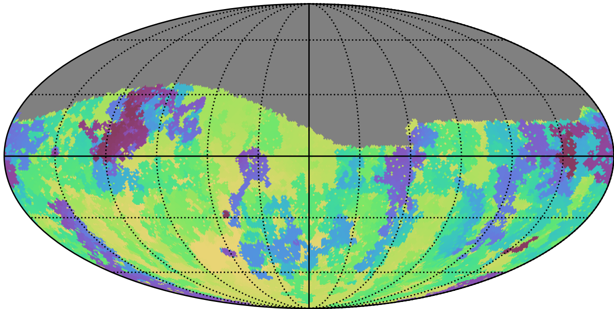
weather_cloudso0v3.4_10yrs Yr 1 g band: Min skyBrightness
