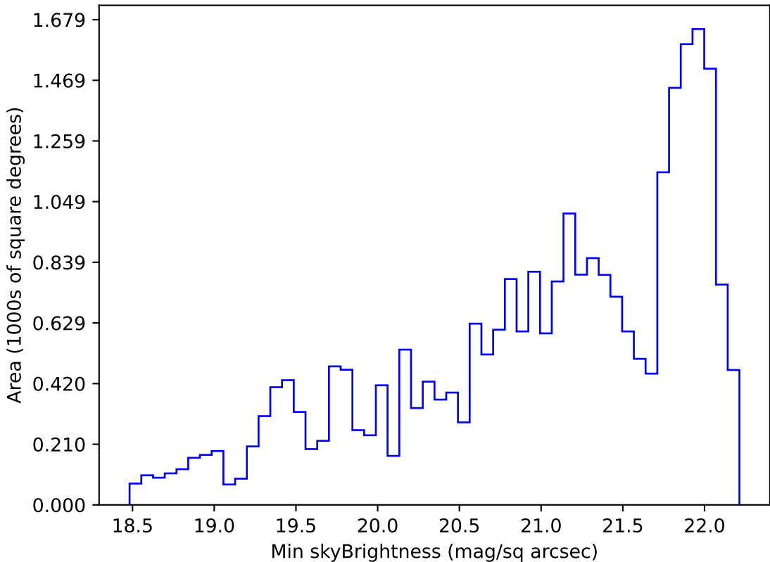
weather_cloudso0v3.4_10yrs Yr 1 g band: Min skyBrightness
