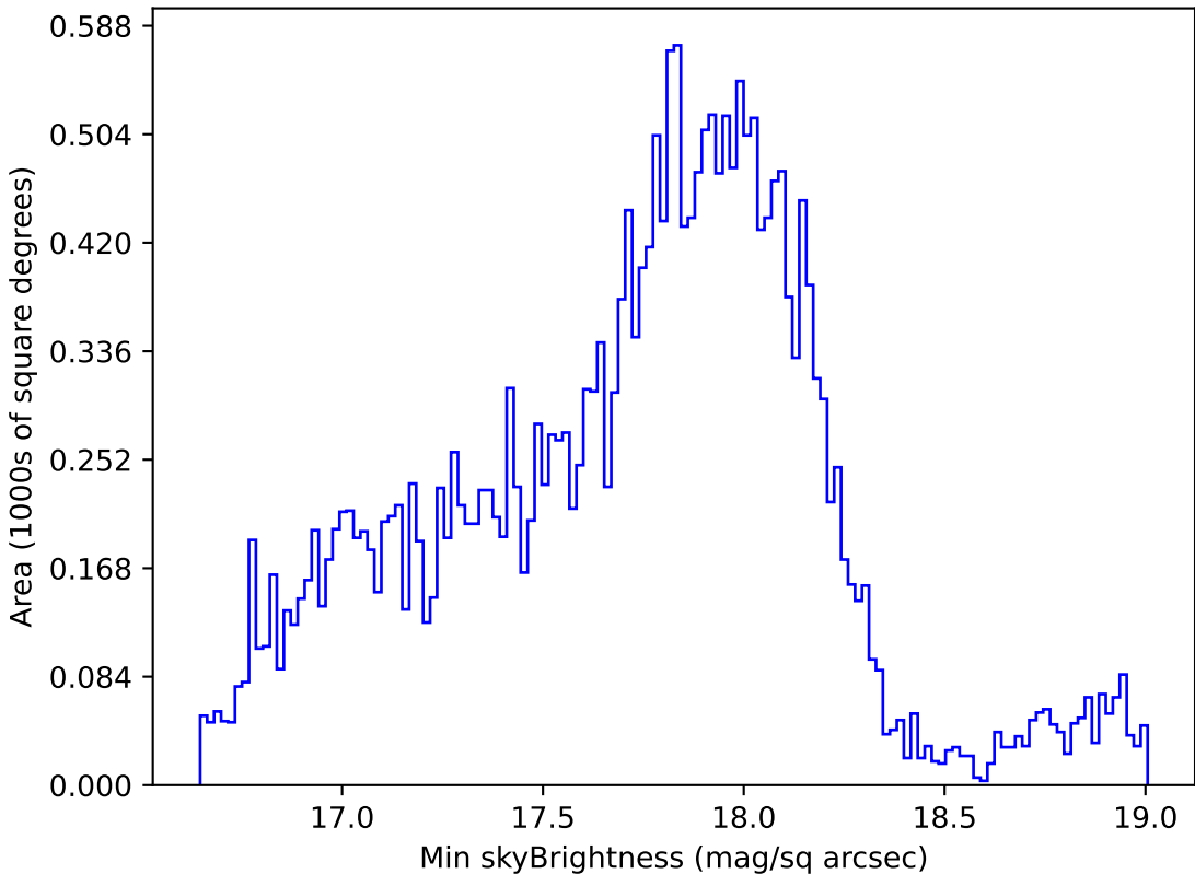
weather_cloudso0v3.4_10yrs Yr 1 all bands: Min skyBrightness
