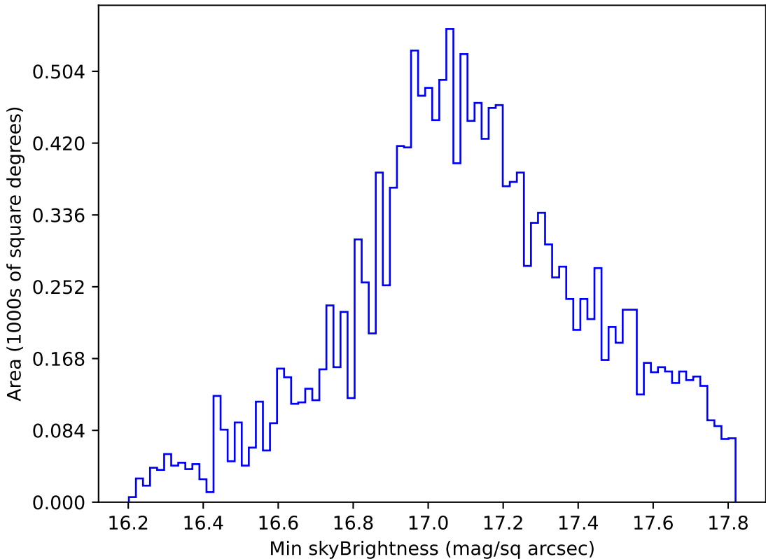
weather_cloudso0v3.4_10yrs WFD y band: Min skyBrightness
