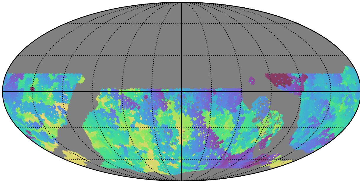
weather_cloudso0v3.4_10yrs WFD u band: Min skyBrightness
