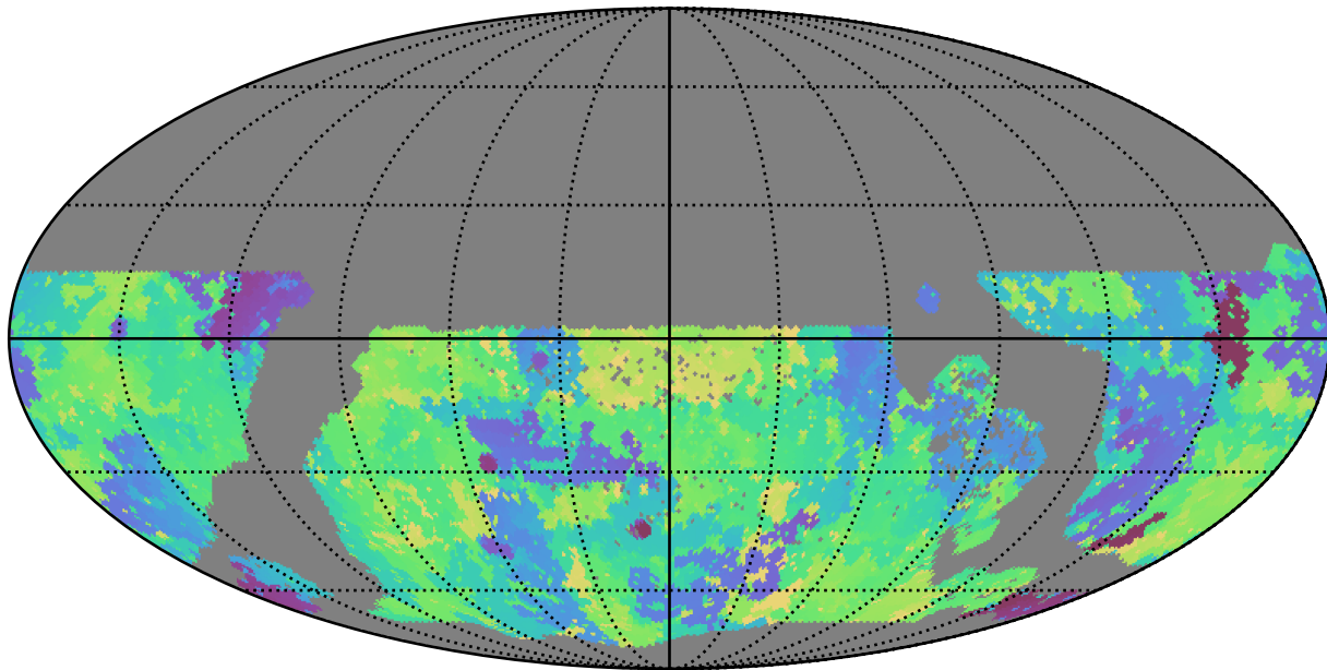
weather_cloudso0v3.4_10yrs WFD g band: Min skyBrightness
