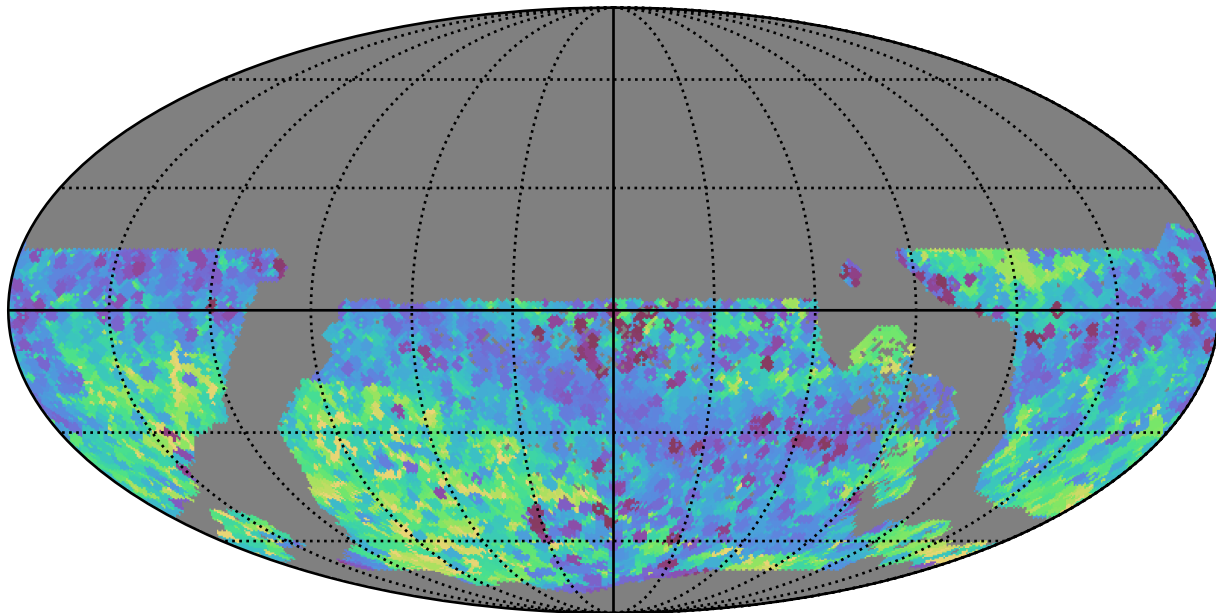
weather_cloudso0v3.4_10yrs WFD all bands: Min skyBrightness
