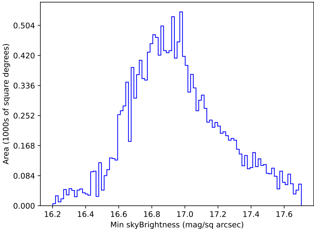
weather_cloudso0v3.4_10yrs WFD all bands: Min skyBrightness
