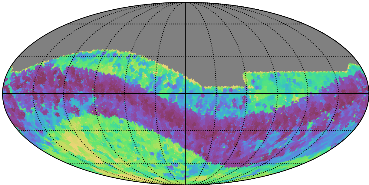
weather_cloudso0v3.4_10yrs All sky z band: Min skyBrightness
