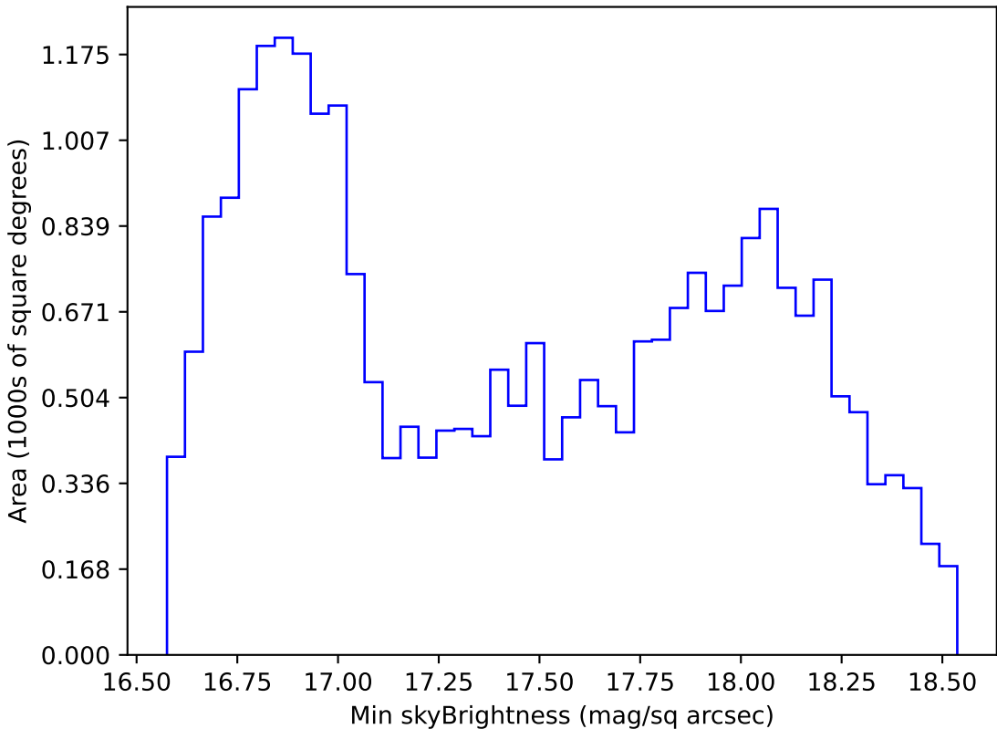
weather_cloudso0v3.4_10yrs All sky z band: Min skyBrightness
