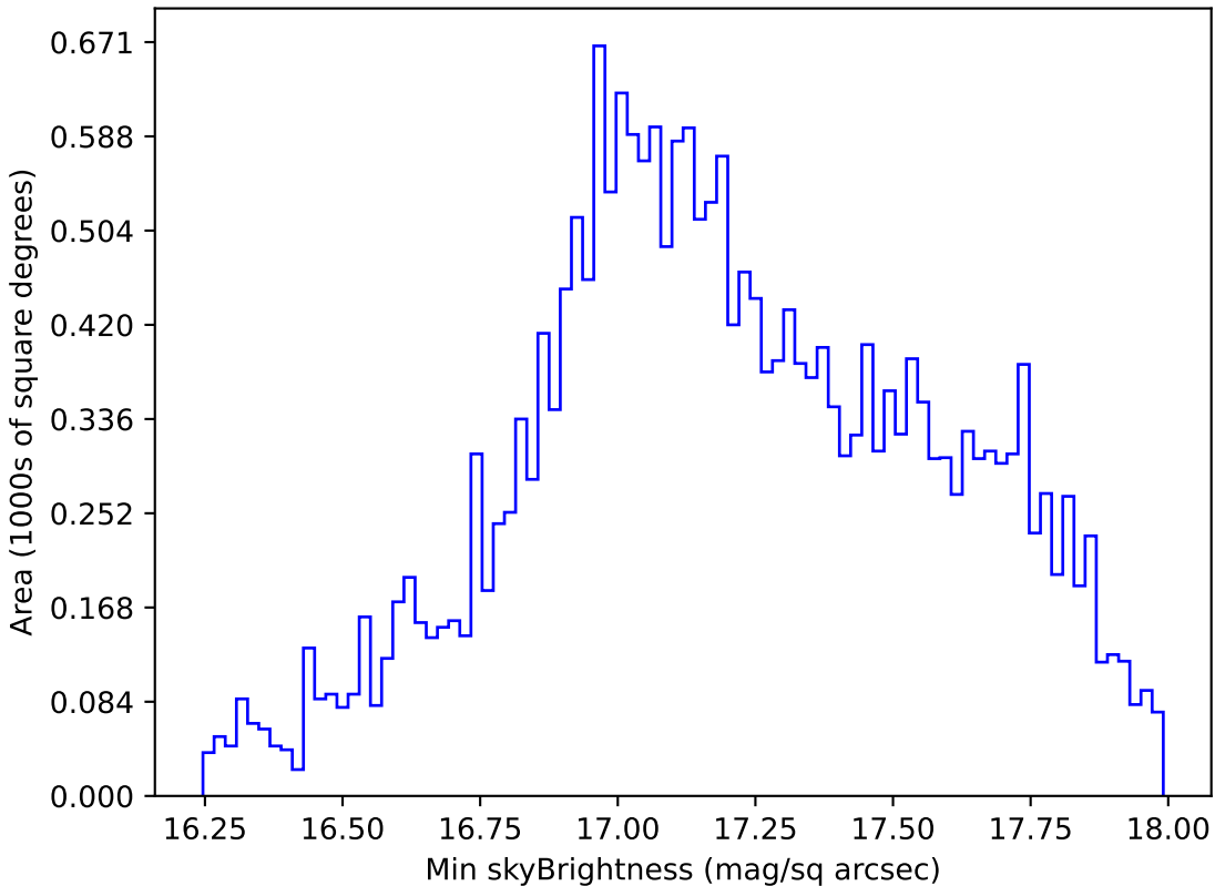
weather_cloudso0v3.4_10yrs All sky y band: Min skyBrightness
