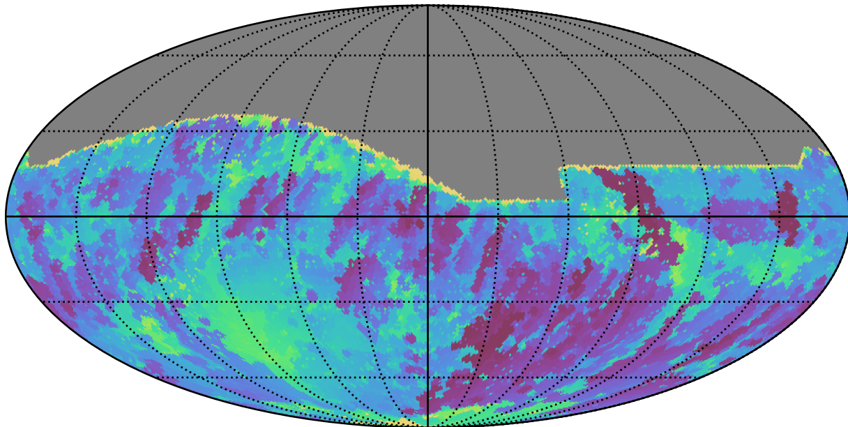
weather_cloudso0v3.4_10yrs All sky r band: Min skyBrightness
