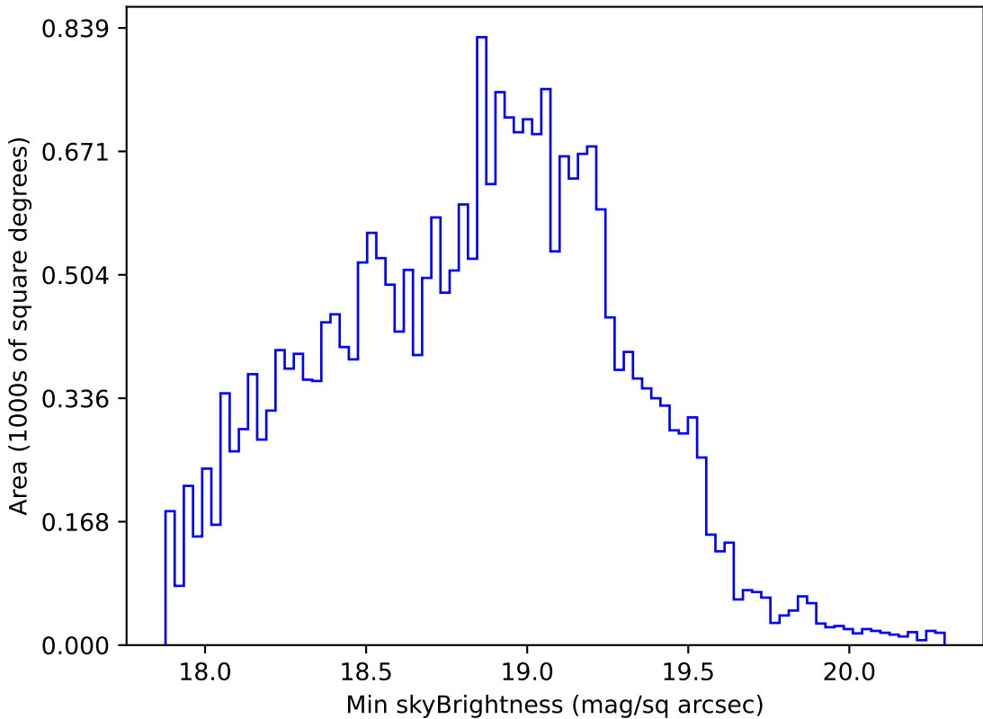
weather_cloudso0v3.4_10yrs All sky r band: Min skyBrightness
