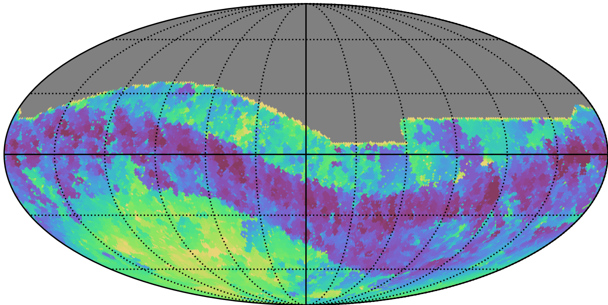
weather_cloudso0v3.4_10yrs All sky i band: Min skyBrightness
