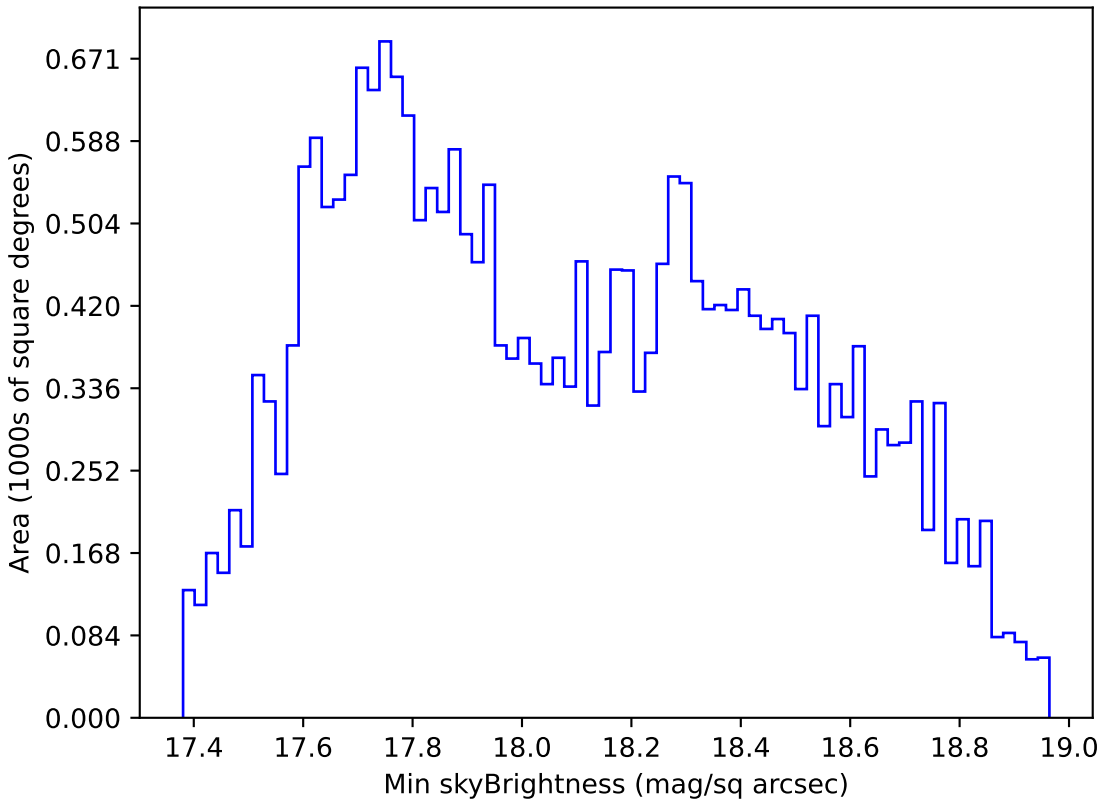
weather_cloudso0v3.4_10yrs All sky i band: Min skyBrightness
