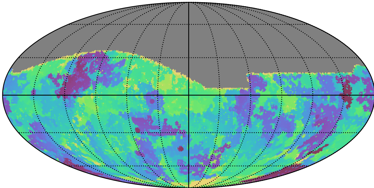
weather_cloudso0v3.4_10yrs All sky g band: Min skyBrightness
