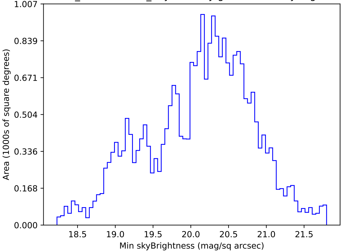
weather_cloudso0v3.4_10yrs All sky g band: Min skyBrightness
