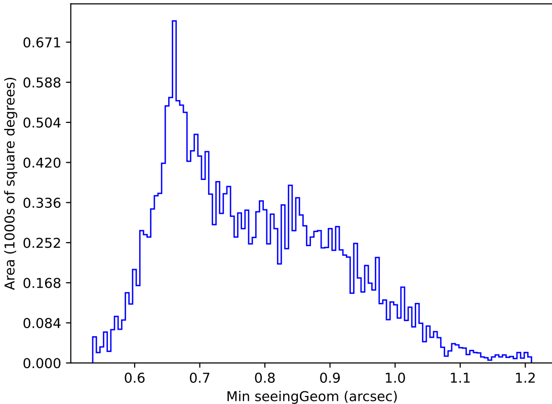
weather_cloudso0v3.4_10yrs Yr 1 u band: Min seeingGeom
