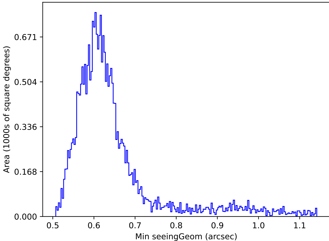
weather_cloudso0v3.4_10yrs Yr 1 r band: Min seeingGeom
