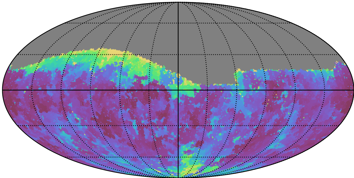
weather_cloudso0v3.4_10yrs Yr 1 g band: Min seeingGeom
