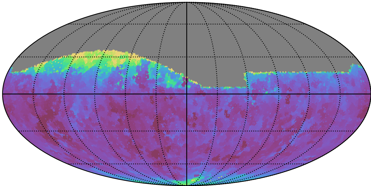
weather_cloudso0v3.4_10yrs Yr 1 all bands: Min seeingGeom
