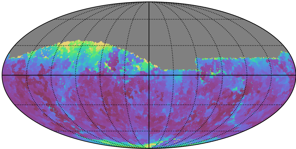
weather_cloudso0v3.4_10yrs Yr 1 z band: Min seeingEff
