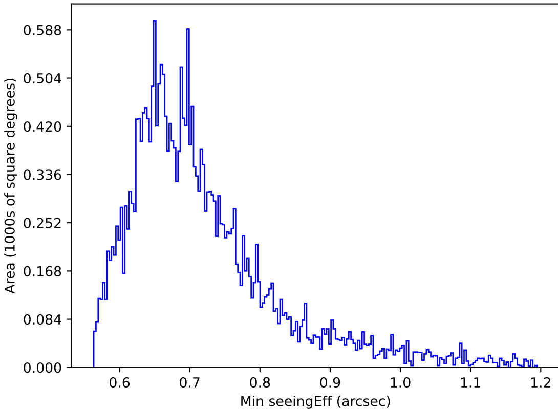
weather_cloudso0v3.4_10yrs Yr 1 z band: Min seeingEff
