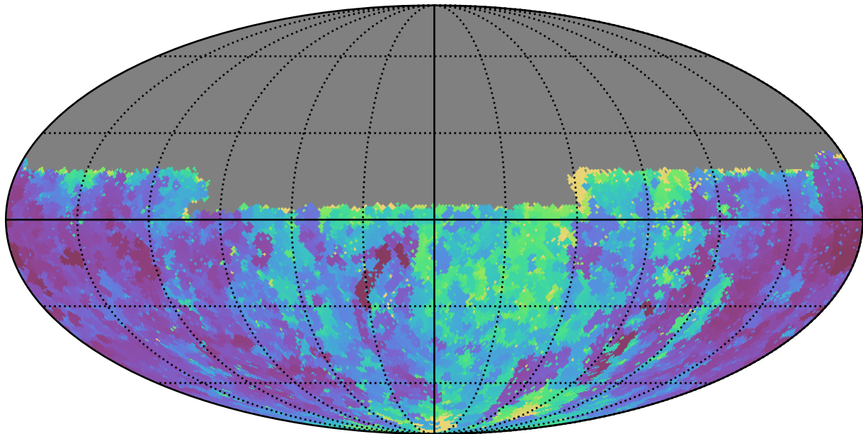
weather_cloudso0v3.4_10yrs Yr 1 u band: Min seeingEff
