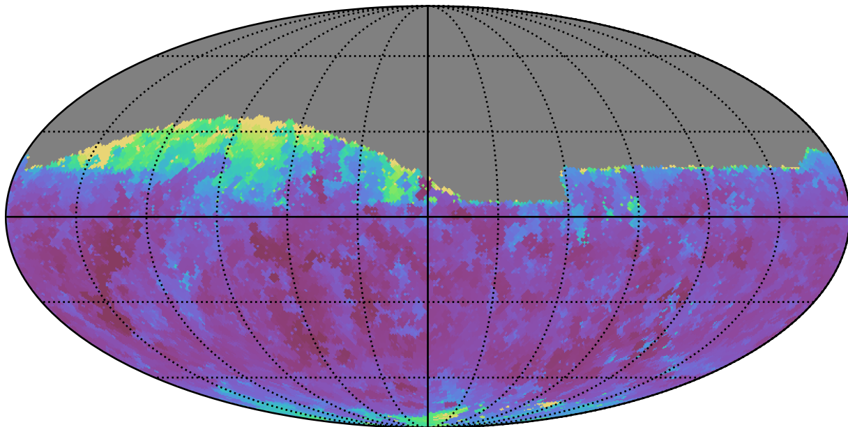
weather_cloudso0v3.4_10yrs Yr 1 i band: Min seeingEff
