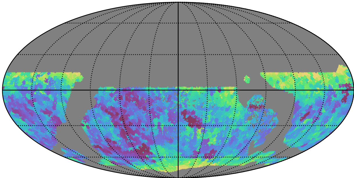
weather_cloudso0v3.4_10yrs WFD z band: Min seeingEff
