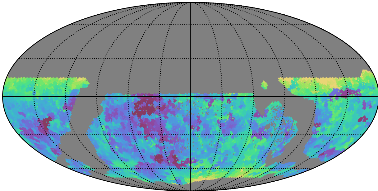
weather_cloudso0v3.4_10yrs WFD r band: Min seeingEff
