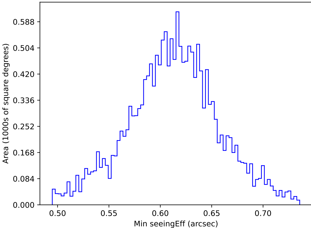
weather_cloudso0v3.4_10yrs WFD r band: Min seeingEff
