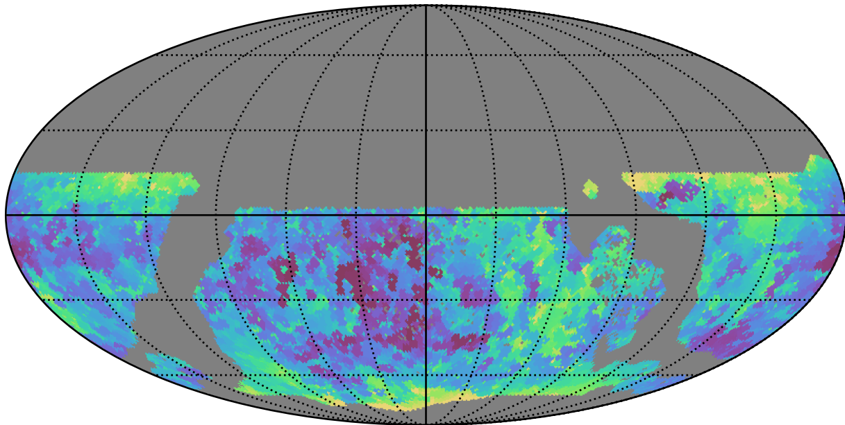
weather_cloudso0v3.4_10yrs WFD g band: Min seeingEff
